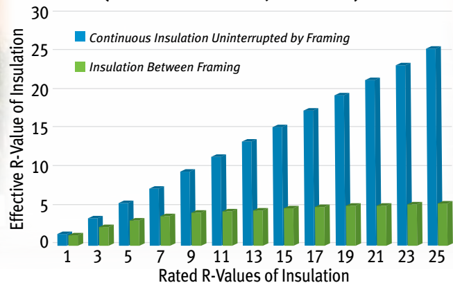
Effective R-Value for Continuous Insulation Uninterrupted by Framing Compared to Installation Between 3.5 inch Metal Studs (from ASRAE 90.1-2007, Table A3.1D)
